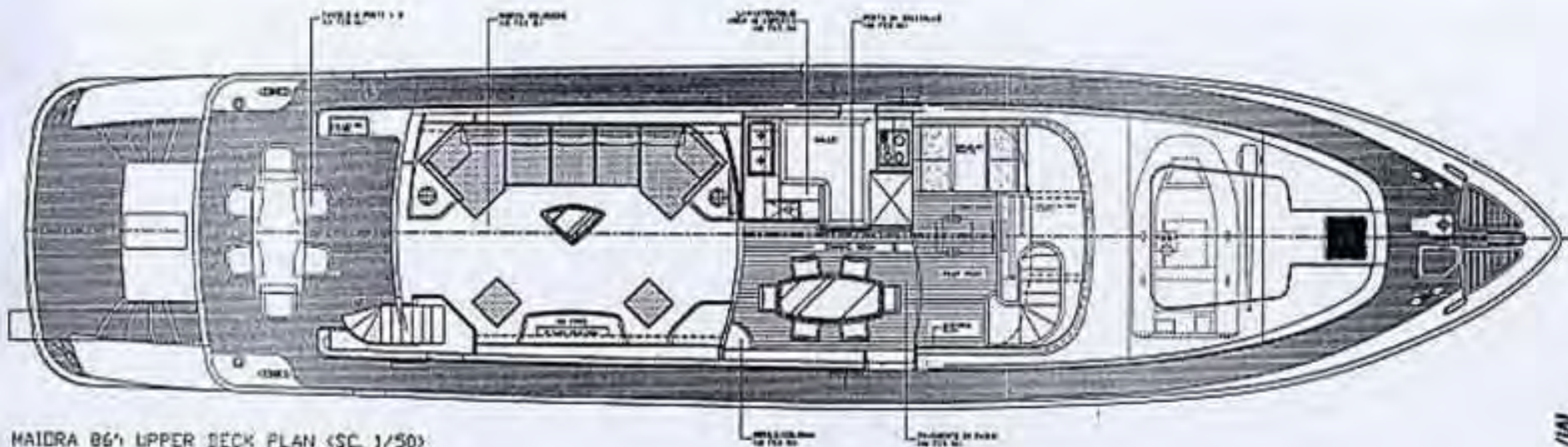
MAIDRA 86' UPPER DECK PLAN (SC. 1/50)
