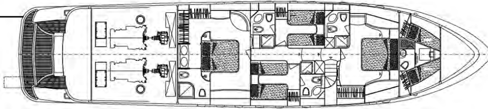
LOWER DECK
