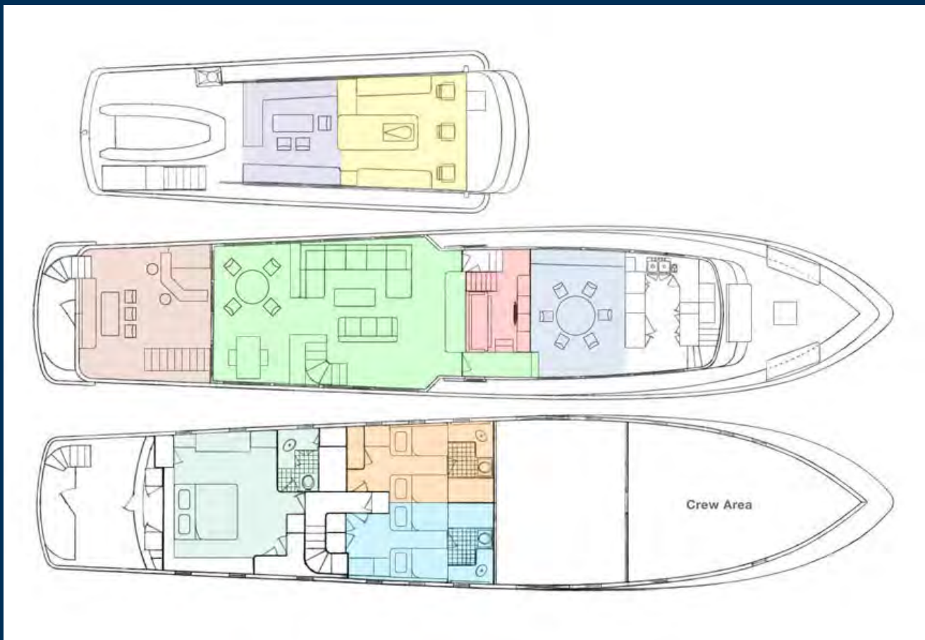
REFLECTIONS Layout
