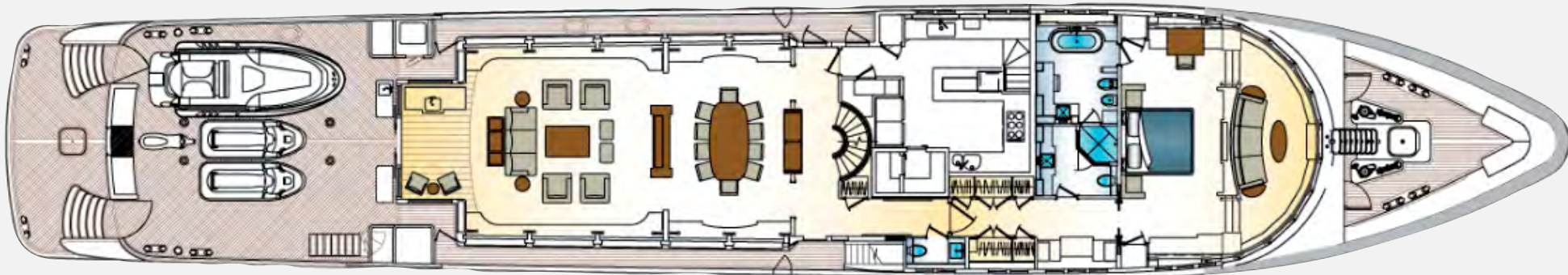
main deck
